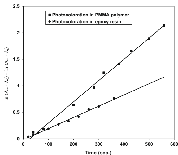
Figure 3 First-order plot of the photocoloration of SO doped in PMMA and epoxy resin.
