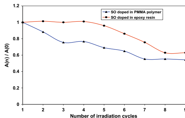
Figure 7 Photochemical fatigue resistance of SO doped in PMMA and epoxy resin polymer films.
