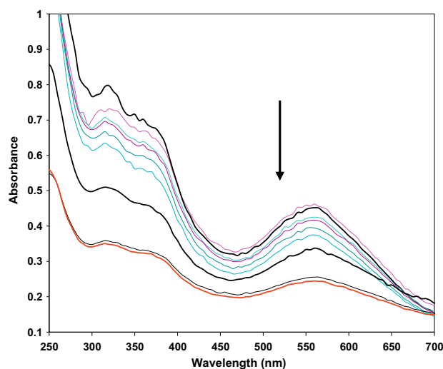
Figure 4 Photobleaching reaction of PMC in PMMA polymer film. The arrow direction indicates the decrease of absorbance with increasing exposure time (s), 0; 20; 100; 120; 200; 240; 280; 340; 560.
