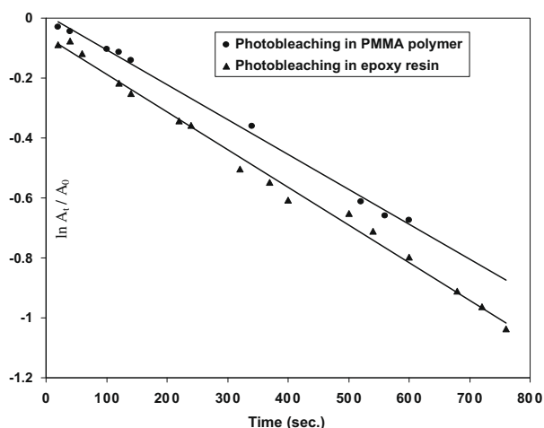
Figure 6 First-order plot of the photobleaching reaction of PMC in PMMA and epoxy resin films.
