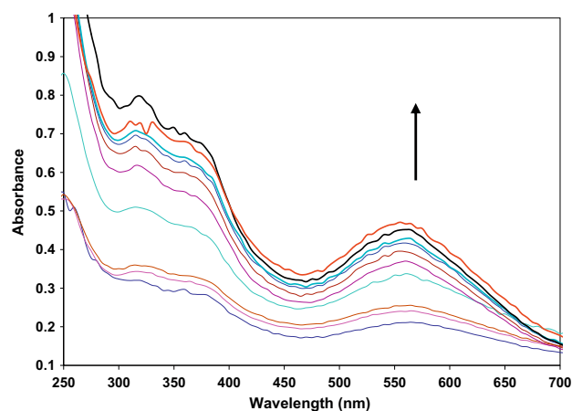
Figure 1 Photocoloration of SO doped in PMMA polymer film. The arrow direction indicates the increase of absorbance with increasing exposure time (s), 0; 20; 40; 100; 120; 140; 200; 240; 280; 340; 520; 560; 600.
