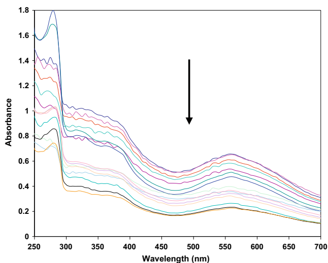
Figure 5 Photobleaching reaction of PMC in epoxy resin film. The arrow direction indicates the decrease of absorbance with increasing exposure time (s), 0; 20; 40; 60; 80; 140; 180; 320; 400; 440; 500; 540; 680; 720.
