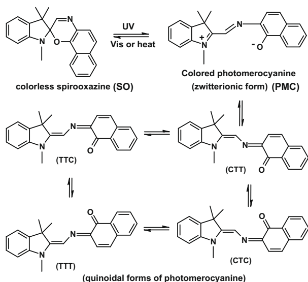
Scheme 1 Photochemical reactions of spiroindolenaphthooxazine.
