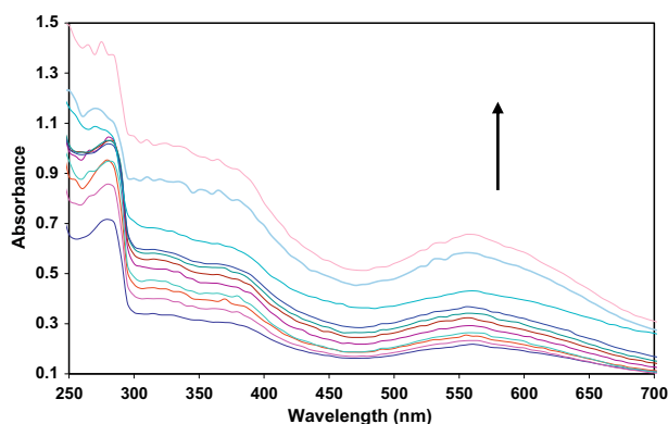
Figure 2 Photocoloration of SO doped in epoxy resin polymer film. The arrow direction indicates the increase of absorbance with increasing exposure time (s), 0; 20; 40; 60; 100; 140; 180; 220; 300; 480; 540.
